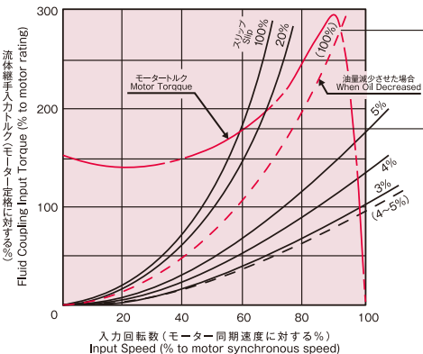
Fig.A Characteristics for input(motor)shaft connecting part.
