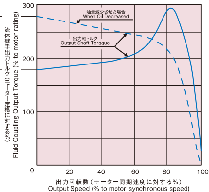
Fig.B Characteristics for output(gear reducer)shaft connecting part.
