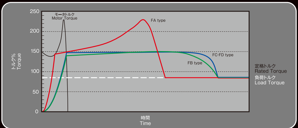
時間軸での性能比較 Characteristics by Time Elapse Axle
